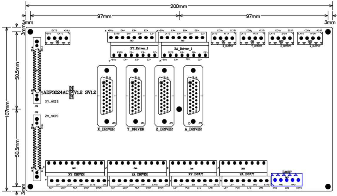
ADP3024ACDIN for JF1,2 (MPC3024AC only)
