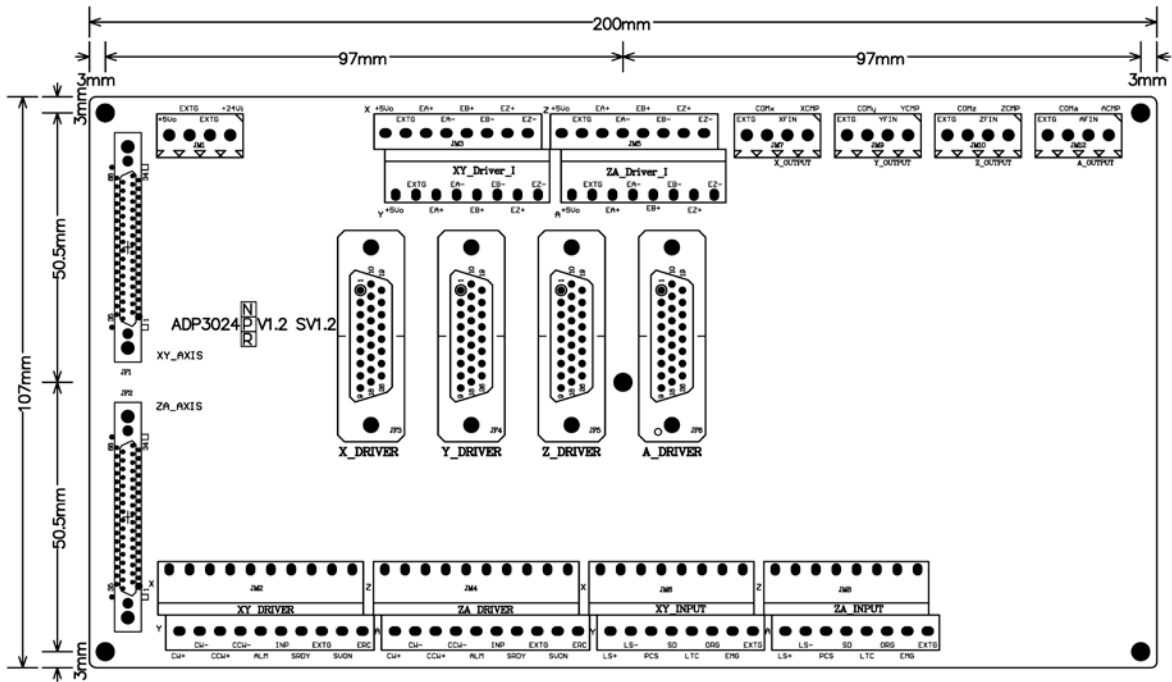
ADP3024DIN for JF1,2
