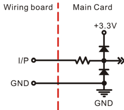
For Pulse Handler Input : PA,PB
