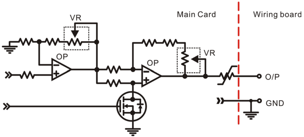
Digital to analog converter (ADP3024ACDIN Only)
