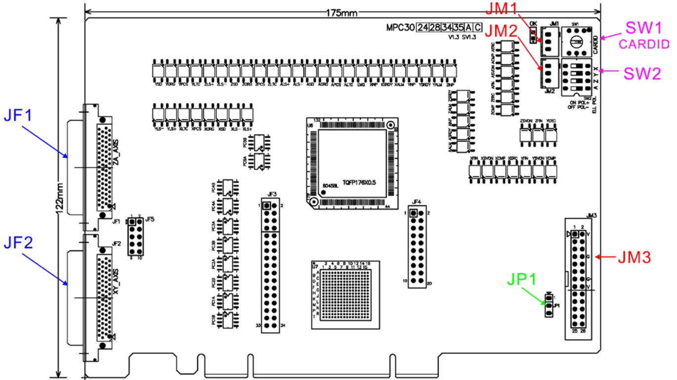
MPC3024AC/ MPC3024A main card
