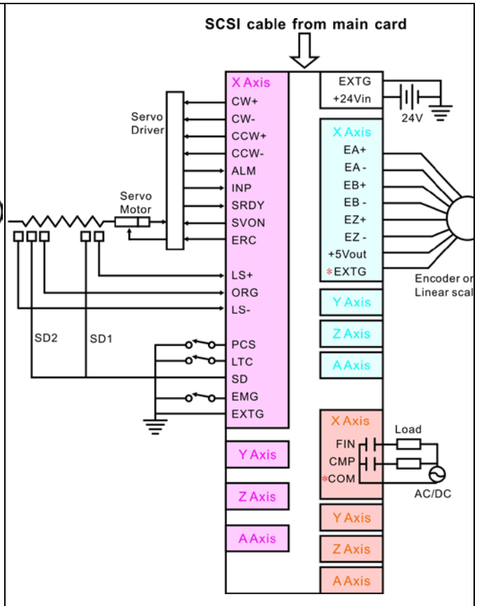
MPC3024A Wiring board with Relay output
