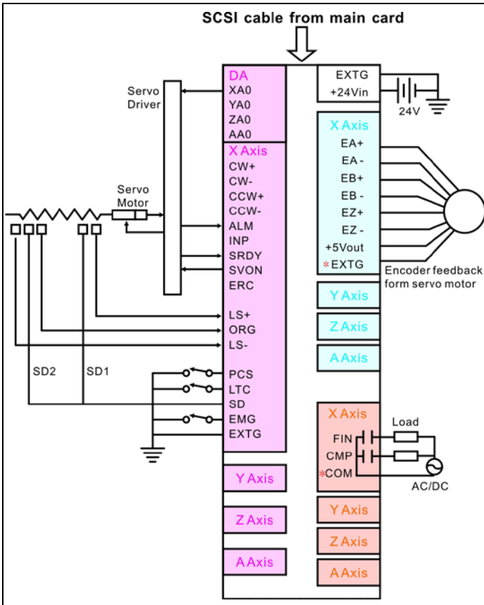
MPC3024AC Wiring board with Relay output
