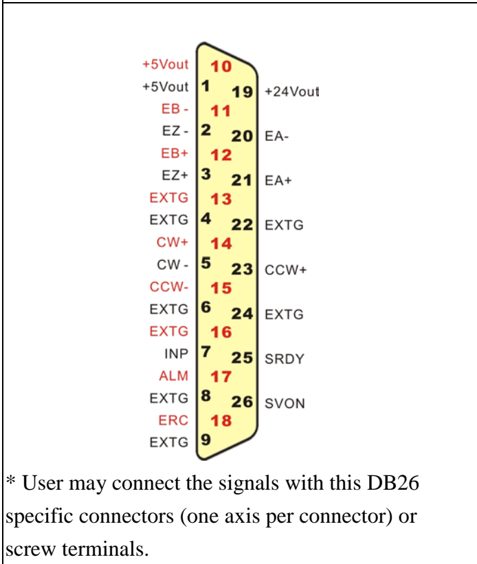
Wiring board DB26 specific connector
